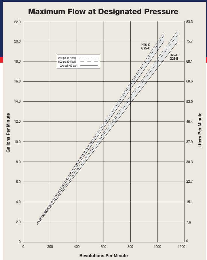
H25/G25 with Cast Iron pump head. Also available in (metallic) Brass, Duplex Alloy 2205, 316L Stainless Steel (with ANSI flanges), 316L Stainless Steel, Hastelloy CW12MW and (non-metallic) Polypropylene and PVDF pump heads.
