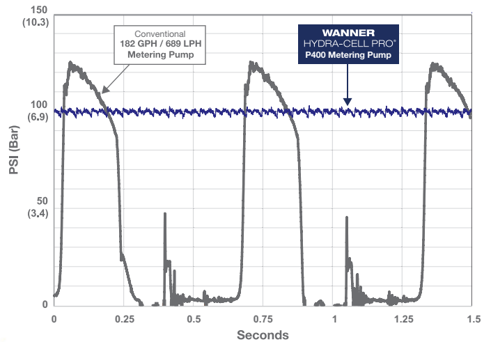
Pulsation Graph Comparison Metering pumps operating without pulsation dampeners Flow rate: 182 gph (689 lph) – Pressure: 100 psi (6.9 bar)
