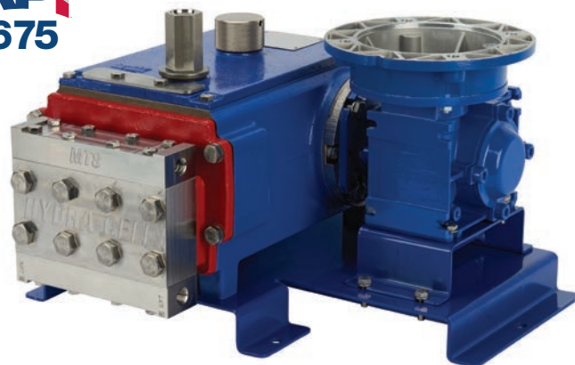
With its multiple-diaphragm design, the MT8 Medium Pressure (above) and MT8 Low Pressure (below) models provide virtually pulse-free flow.
