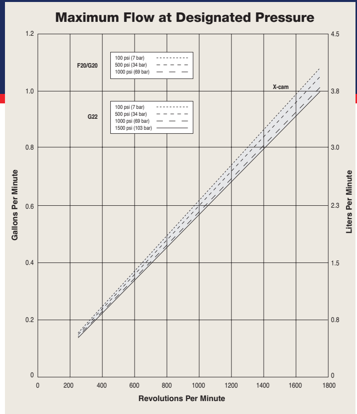
F20/G20 close-coupled for 56C frame or IEC 80 footed motors shown. G22 models to IEC 80 - 90 B5 frame motors. Pump head materials include (metallic) Brass, 316L Stainless Steel and Hastelloy C and (non-metallic) Polypropylene and PVDF.
