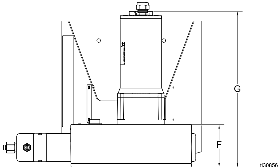
FIG. 13 G-Chem Pump Dimensions
